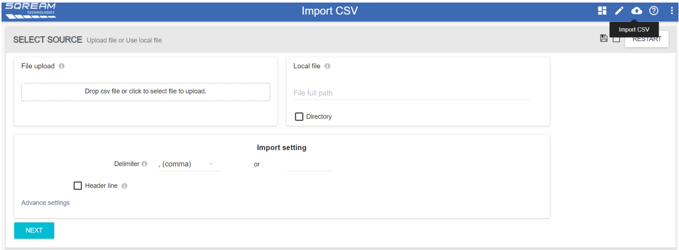
Figure 7. Import CSV
