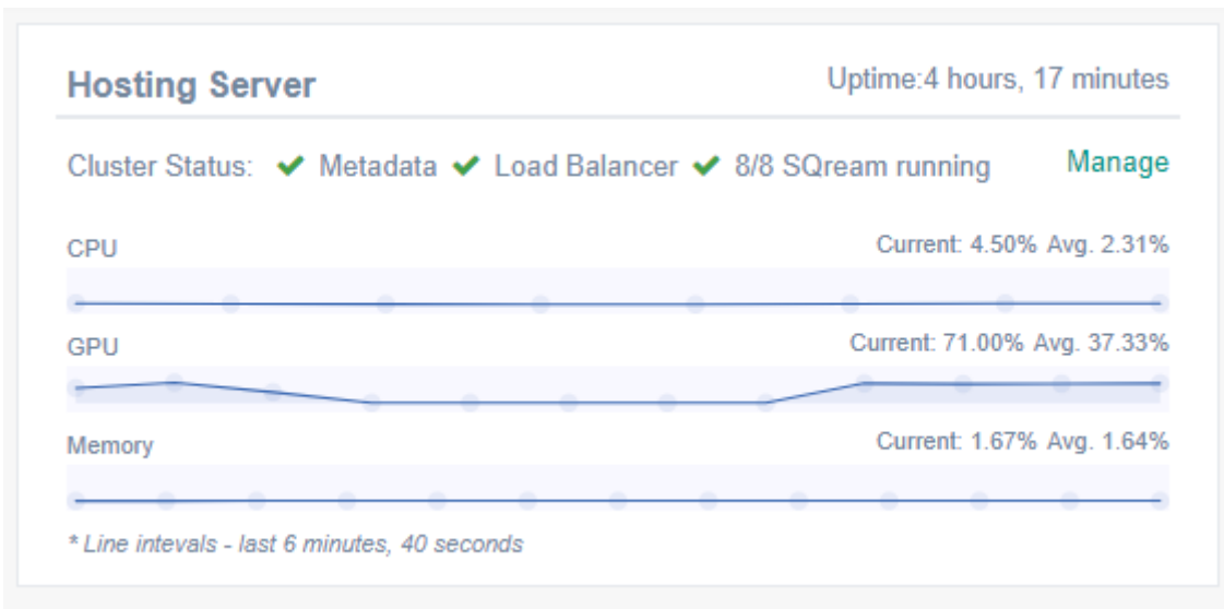
Figure 2. Hosting Panel
