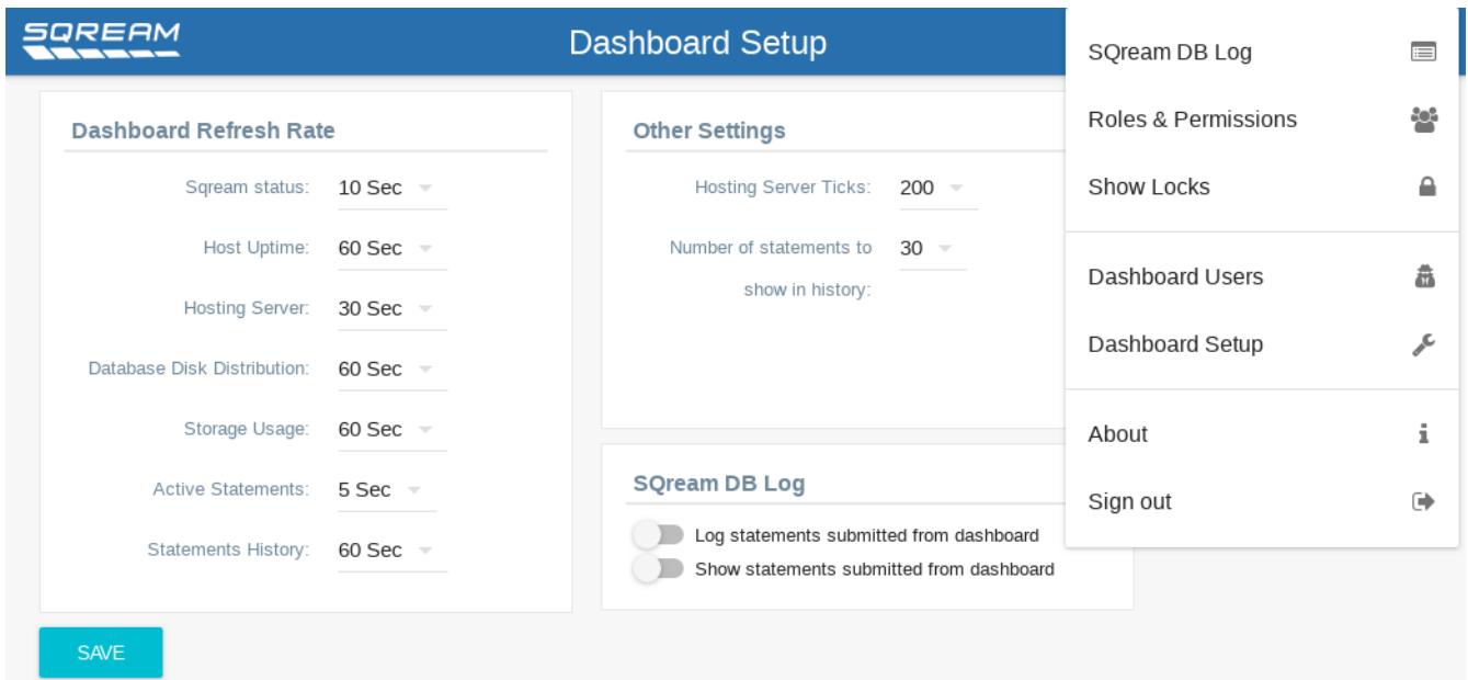
Figure 12. Dashboard Setup
